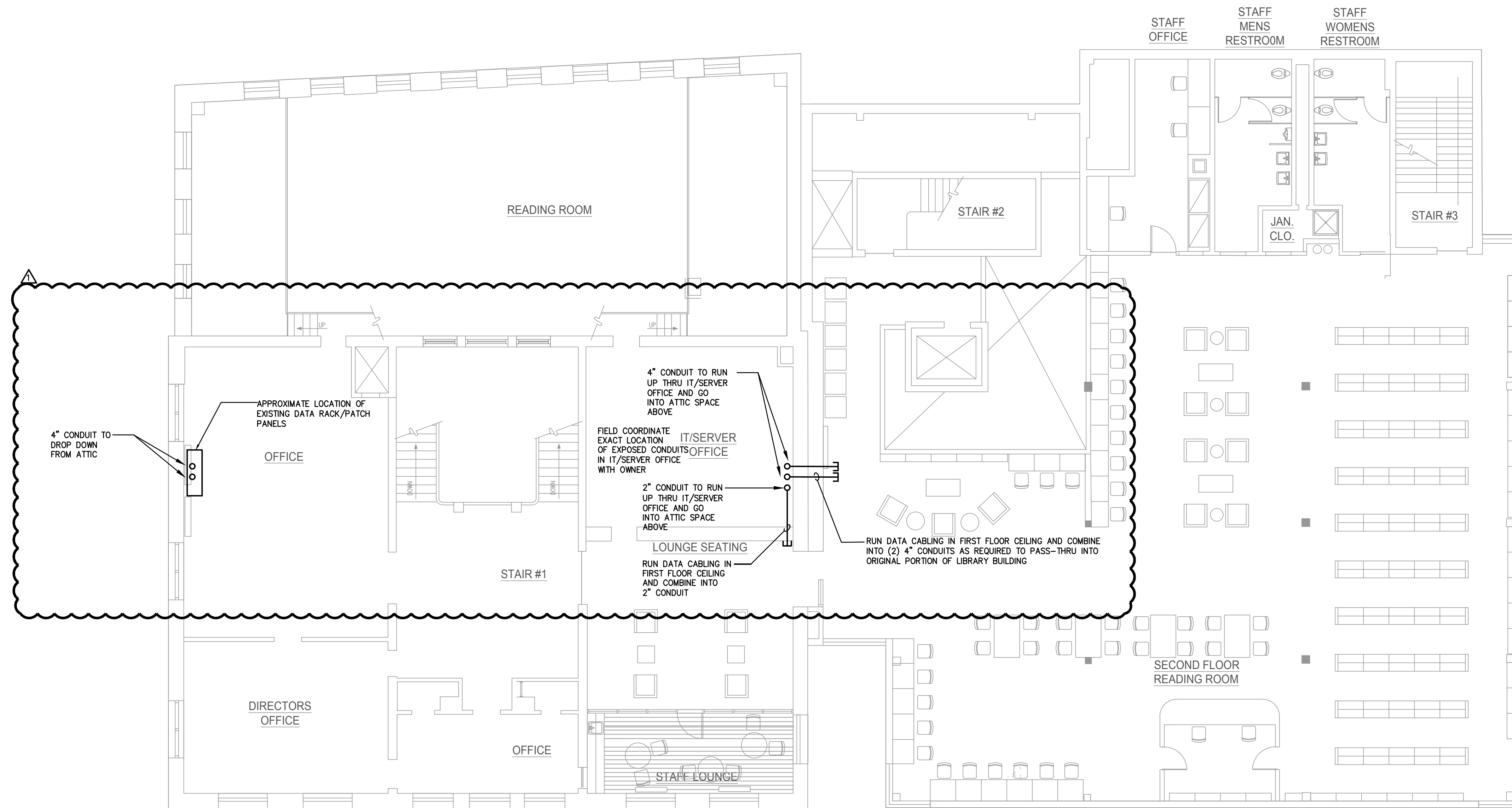
1 SECOND FLOOR PLAN - ELECTRICAL E102 SCALE 1/4" = 1'-0"
