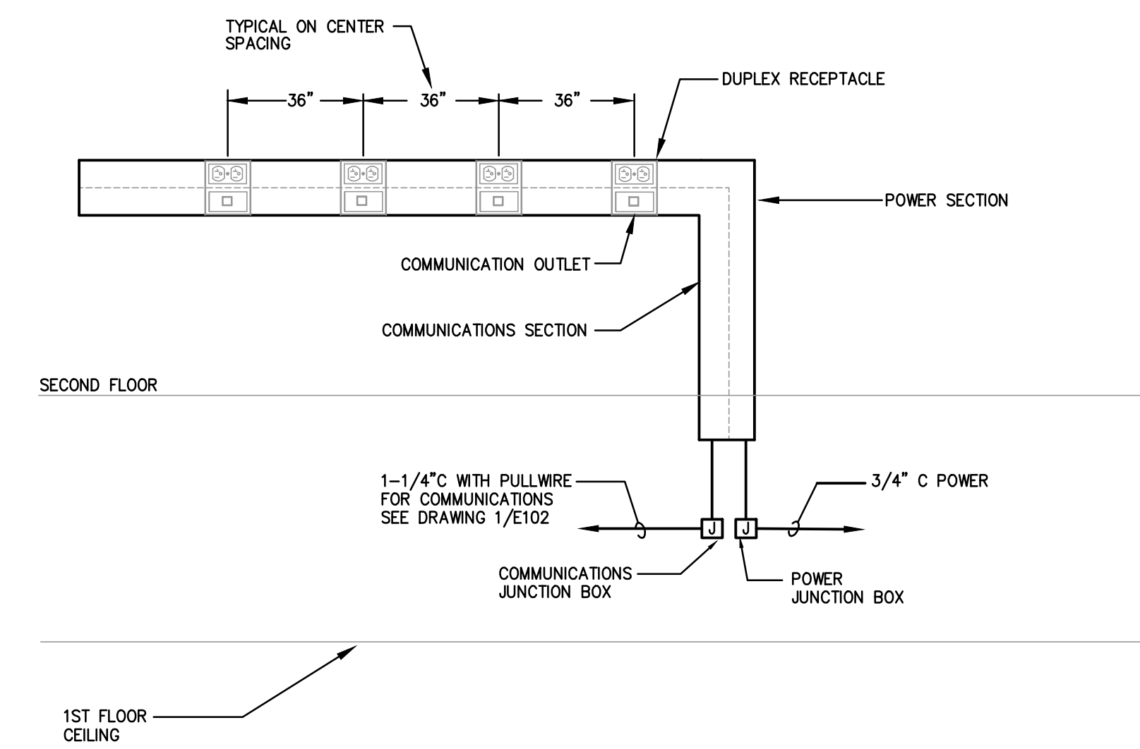
2 TYPICAL WALL MOUNTED MULTI-OUTLET ASSEMBLY ARRANGEMENT DETAIL E102 NOT TO SCALE
