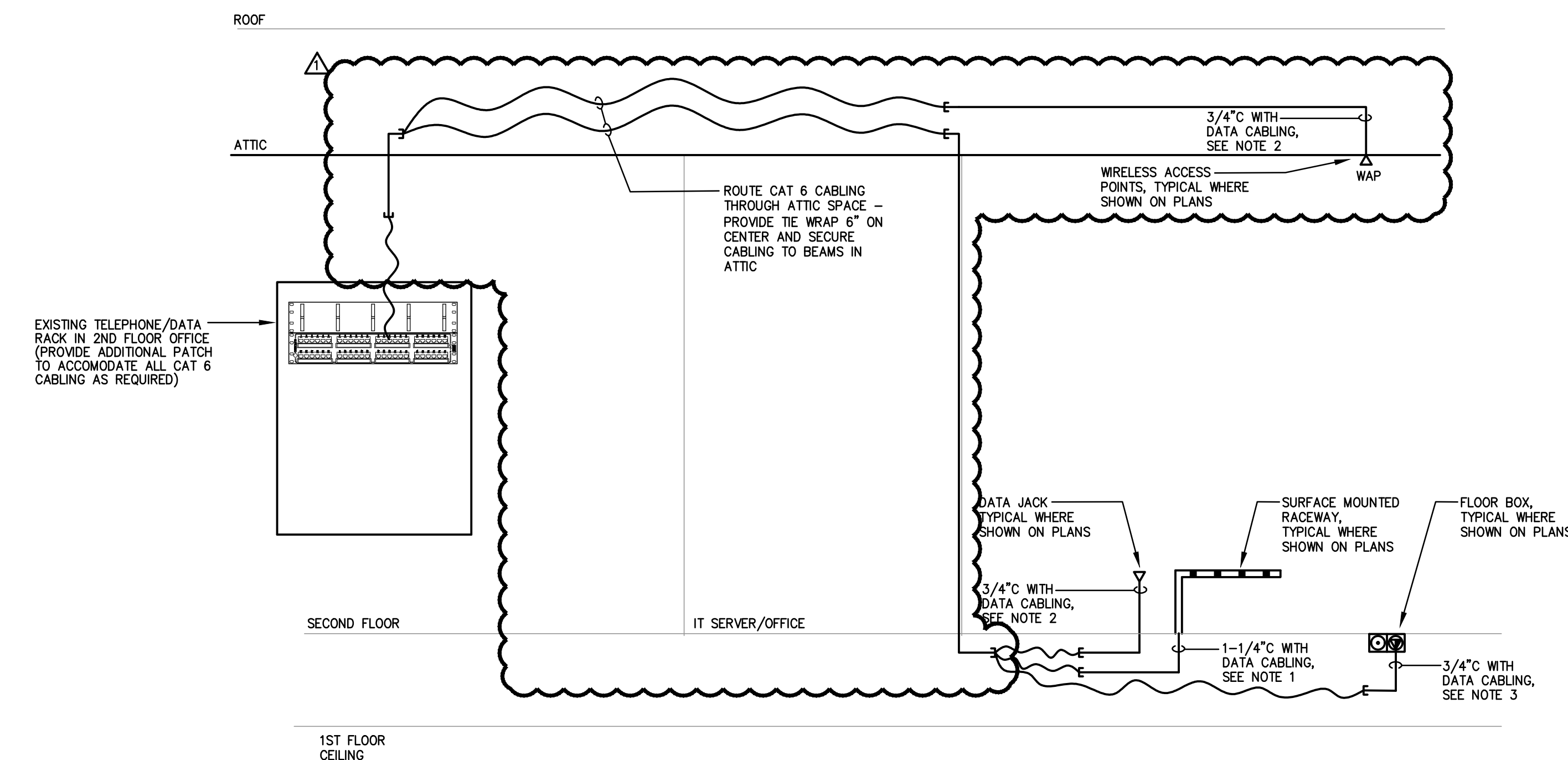
3 TELEPHONE/DATA RISER DIAGRAM E102 SCHEMATIC
